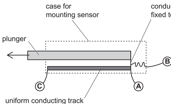
structure of position sensor
